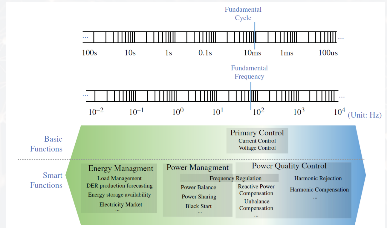
Functions of a smart microgrid.
